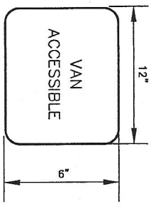
SIGN R7-8V WHITE LEGEND ON BLUE REFLECTORIZED BACKGROUND
