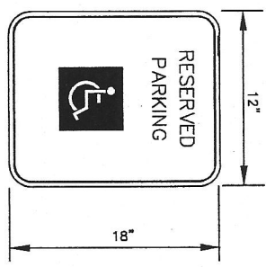
SIGN R7-8 LEGEND & BORDER-GREEN WHITE SYMBOL ON BLUE BACKGROUND BACKGROUND-WHITE
