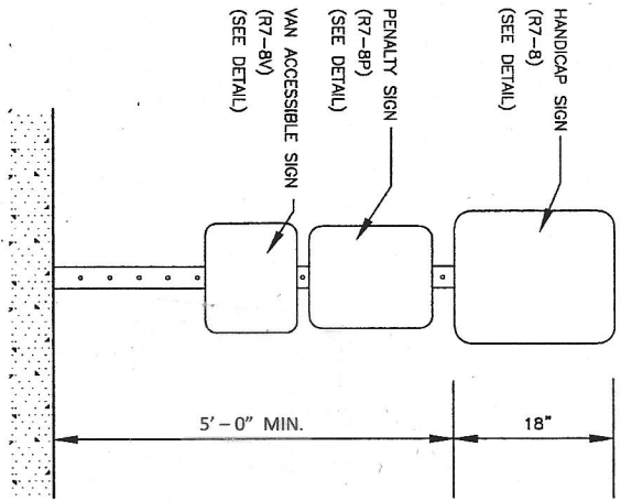
SIGN R7-8 LEGEND & BORDER-GREEN WHITE SYMBOL ON BLUE BACKGROUND BACKGROUND-WHITE
